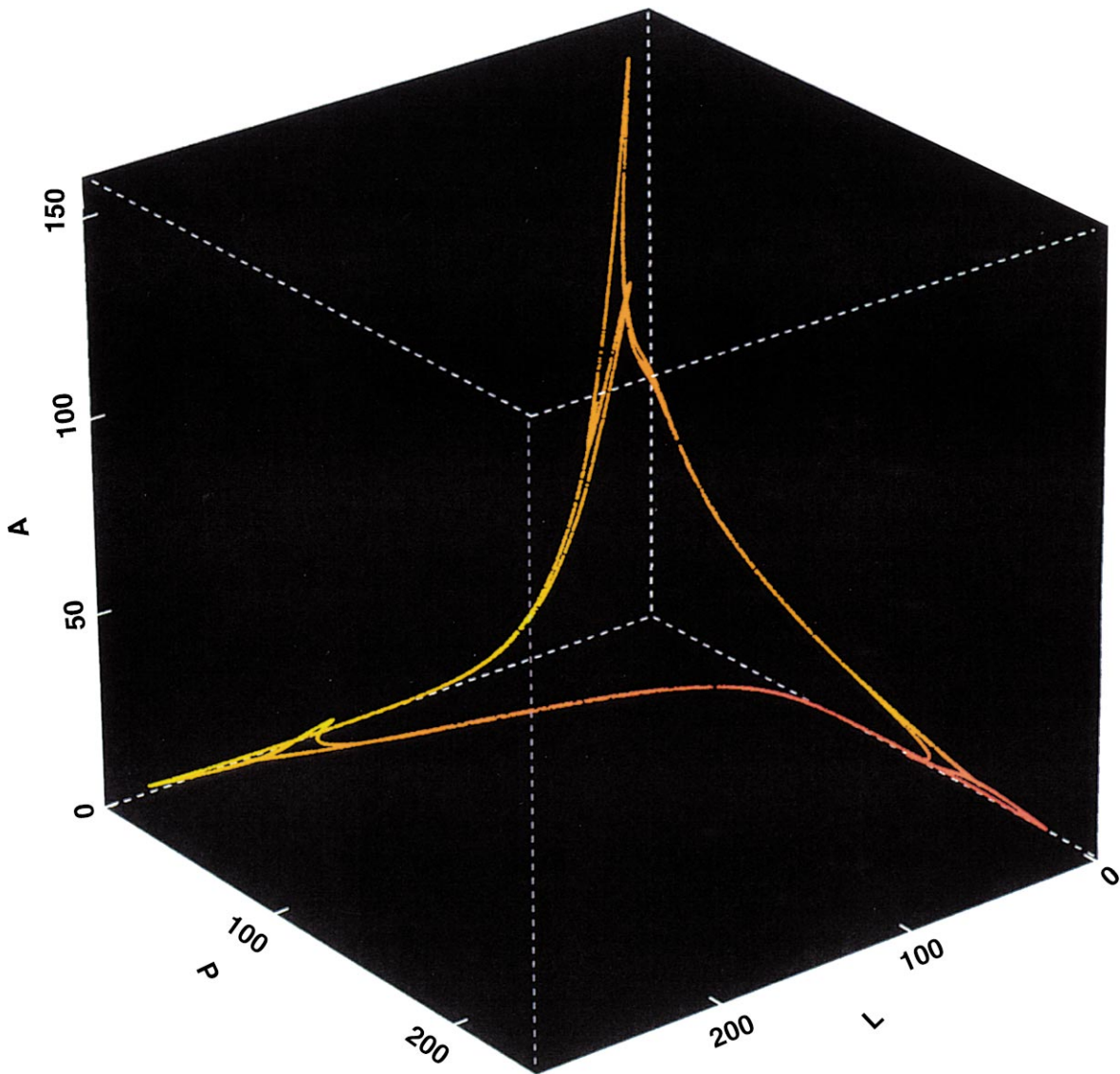
Fig. 6. The chaotic attractor for the deterministic LPA model (1) with \mu_a = 0.96 , c_{pa} = 0.35 and other parameters given in Table 1. This “tangled triangle” attractor is color-coded using the log magnitude of the largest eigenvalue of the Jacobian matrix (the “one-step local Lyapunov exponent”), which ranges from -1.031 (yellow) to 3.9520 (red).
