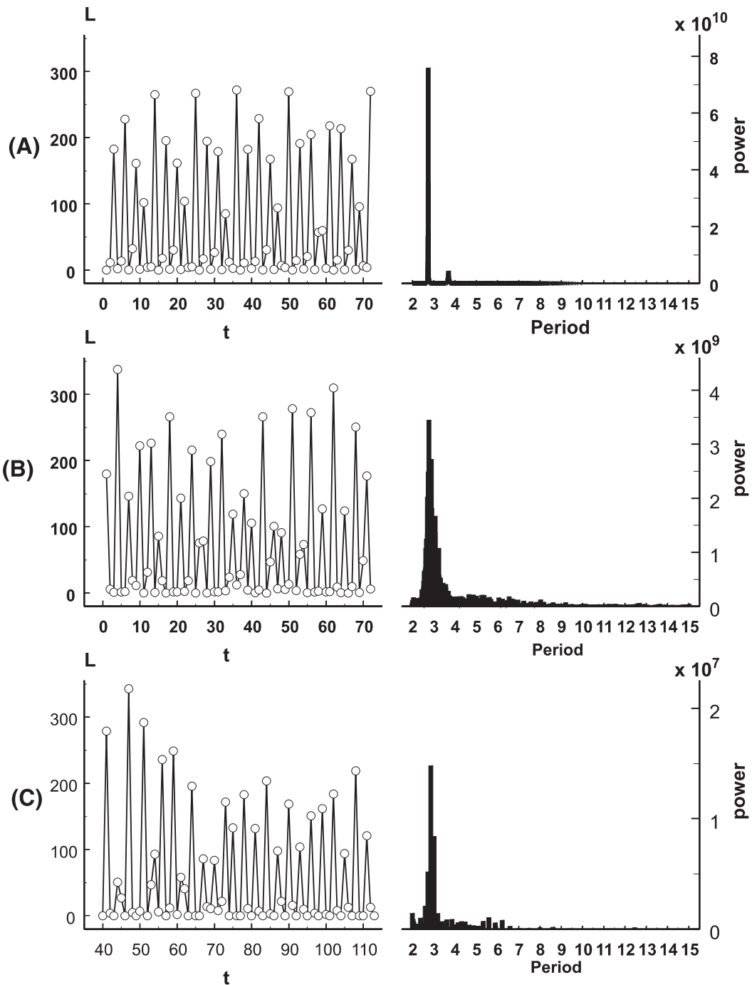
Fig. 12. Graph (A) shows the L component of an orbit on the chaotic attractor of the deterministic model (1) and its power spectrum. Graphs (B) show the same for an orbit of the demographic noise model (2). Graphs (C) show the L component of one replicate of the experimental data for treatment c_{pa} = 0.35 and its power spectrum.
