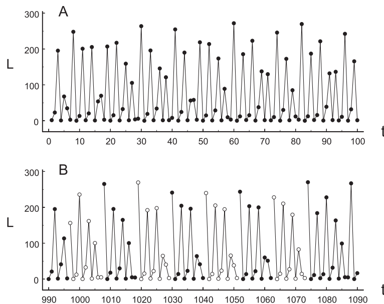
Fig. 11. In graph (A) the L component of a portion of a 10,000-point orbit on the chaotic attractor of the deterministic model (1) shows frequent patterns similar to those of the saddle 11-cycle in Fig. 9. In graph (B) is seen a portion of the orbit during which the pattern is repeated many times in sequence.
