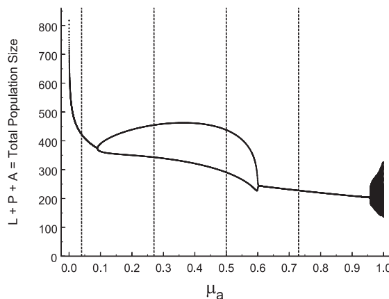
Fig. 1. A bifurcation diagram is shown for the deterministic LPA model (1) using the parameter \mu_a . The other model parameter values are b = 7.483 , \mu_1 = 0.2670 , c_{ca} = 0.009170 , c_{cl} = 0.01200 , c_{pa} = 0.004139 . The vertical dashed lines indicate those \mu_a values at which laboratory experiments were performed [8,9].
