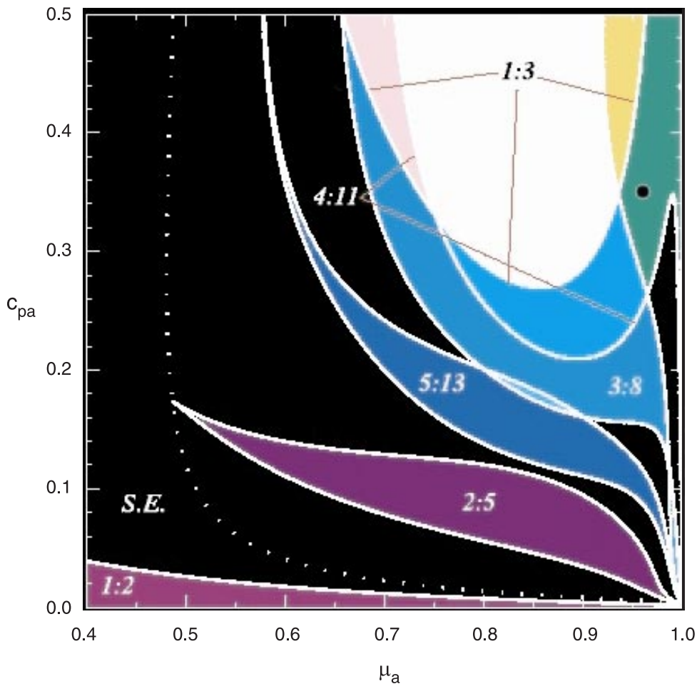
Fig. 10. Selected Arnold's tongues and their rotation numbers are shown in the (\mu_a, c_{pa}) -plane for the LPA model (1) with parameters given in Table 1. Globally stable, positive equilibria occur in the region marked S.E. Invariant loop bifurcations occur when the boundary of the S. E. region denoted by the dotted line is crossed. Period doubling bifurcations to a 2-cycle occur when leaving the SE region along the common boundary with the region marked 1:2. The experimental treatment with \mu_a = 0.96 and c_{pa} = 0.35 (denoted by the black dot) lies in the tongue of 11-cycles with rotation number 4:1.
